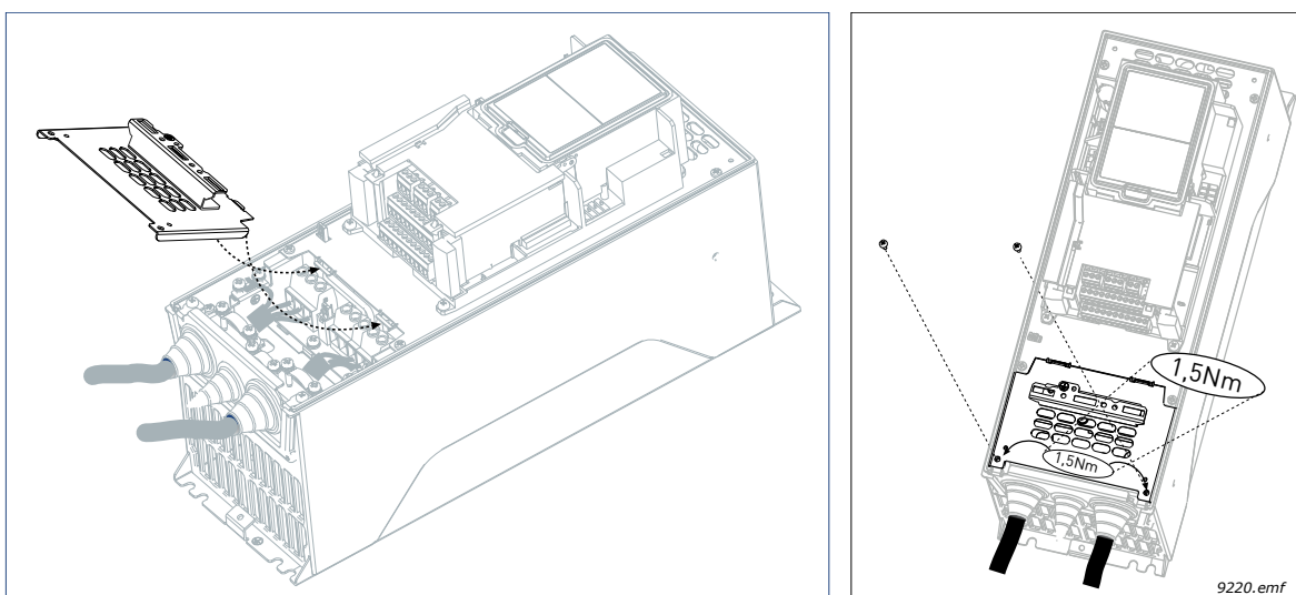
Figure 31. Re-mounting of cover components
